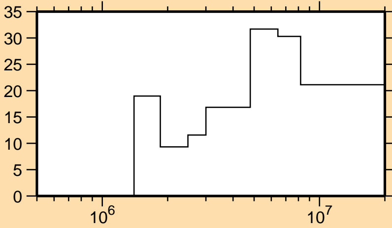
\Delta\sigma/\sigma vs. E for ^{58}\text{Ni}(n,n_1)
