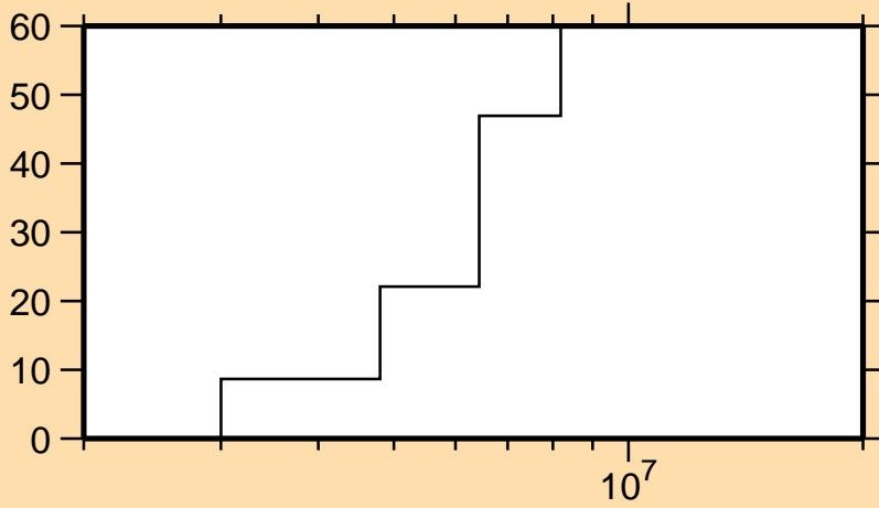
\Delta\sigma/\sigma vs. E for ^{58}\text{Ni}(n,n_6)
