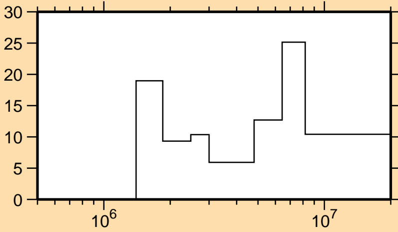
\Delta\sigma/\sigma vs. E for ^{58}\text{Ni}(n,\text{inel.})
