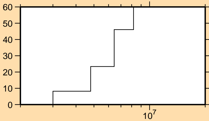
\Delta\sigma/\sigma vs. E for ^{58}\text{Ni}(n,n_{11})
