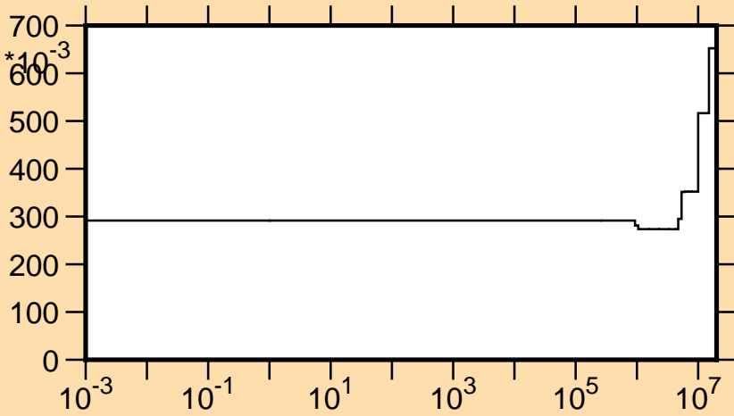
\Delta v/v vs. E for ^{241}\text{Pu} (total \nu )
