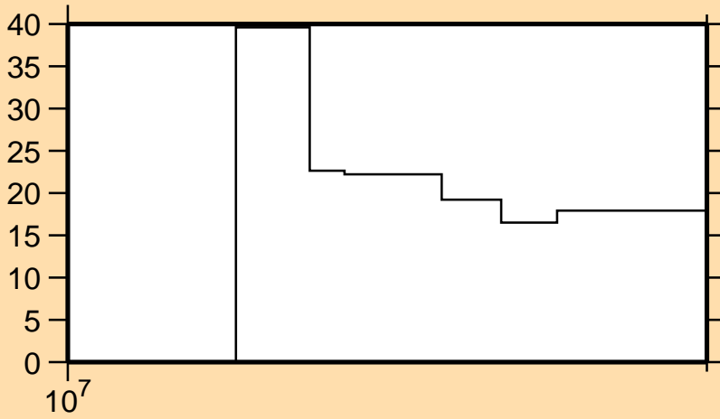
\Delta\sigma/\sigma vs. E for ^{60}\text{Ni}(n,t)
