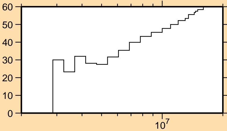
\Delta\sigma/\sigma vs. E for ^{60}\text{Ni}(n,n_6)
