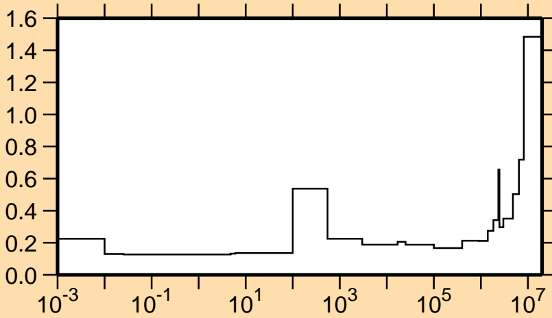
\Delta v/v vs. E for ^{233}\text{U} (prompt \nu )
