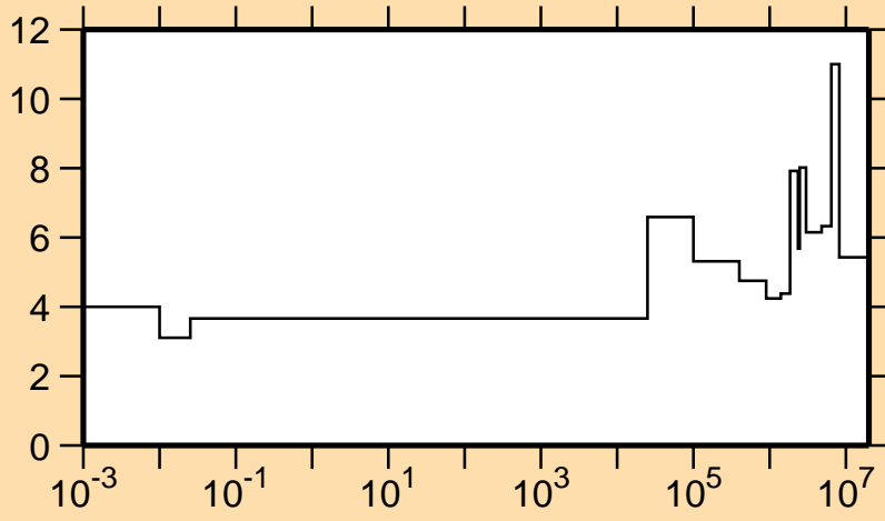
\Delta v/v vs. E for ^{233}\text{U} (delayed \nu )
