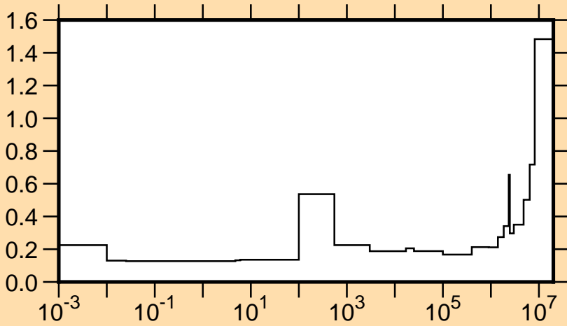
\Delta v/v vs. E for ^{233}\text{U} (total \nu )
