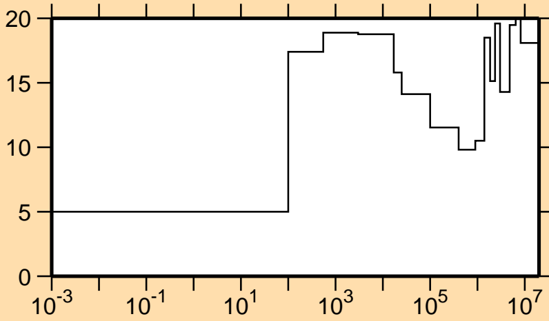
\Delta\sigma/\sigma vs. E for ^{90}\text{Zr}(n,\gamma)
