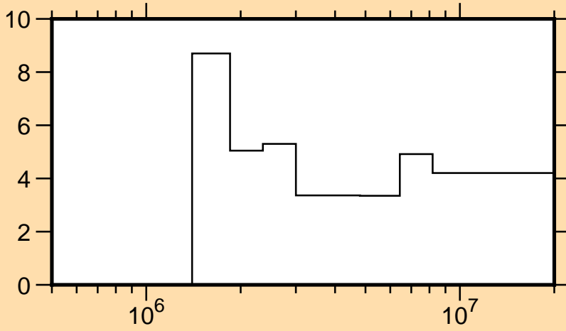
\Delta\sigma/\sigma vs. E for ^{90}\text{Zr}(n,\text{inel.})
