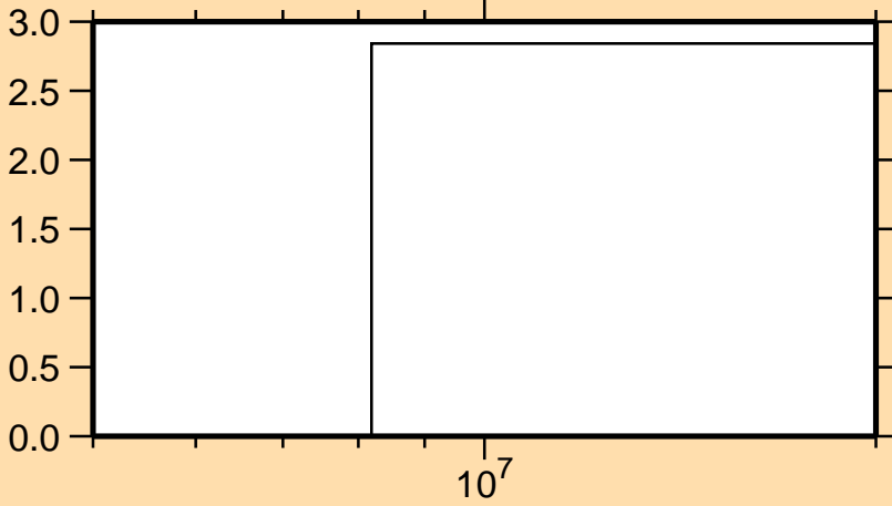
\Delta\sigma/\sigma vs. E for ^{90}\text{Zr}(n,2n)
