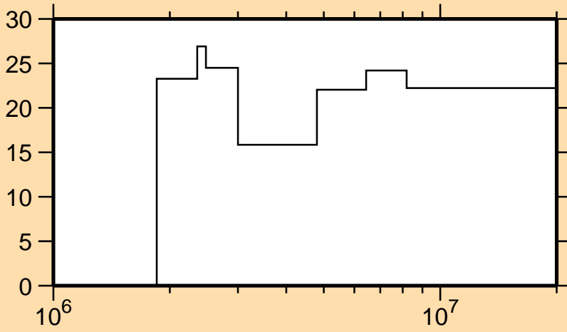
\Delta\sigma/\sigma vs. E for ^{46}\text{Ti}(n,n_2)
