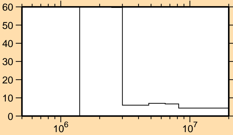
\Delta\sigma/\sigma vs. E for ^{46}\text{Ti}(n,p)
