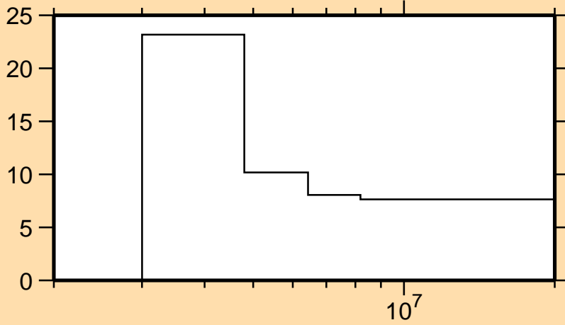
\Delta\sigma/\sigma vs. E for ^{46}\text{Ti}(n,n\text{cont.})
