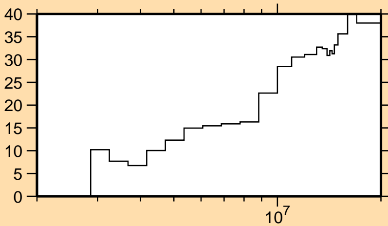
\Delta v/v vs. E for ^{58}\text{Ni}(\text{mt854})
