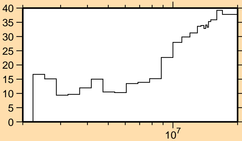
\Delta\sigma/\sigma vs. E for ^{58}\text{Ni}(n,n_2)
