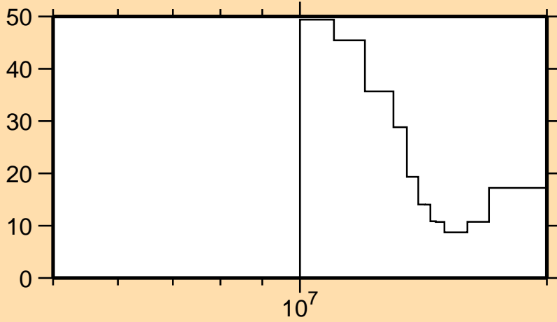
\Delta\sigma/\sigma vs. E for ^{47}\text{Ti}(n,np)
