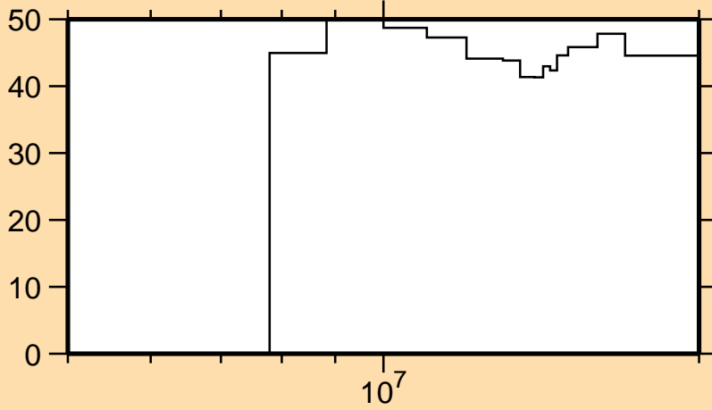
\Delta\sigma/\sigma vs. E for ^{47}\text{Ti}(n,d)
