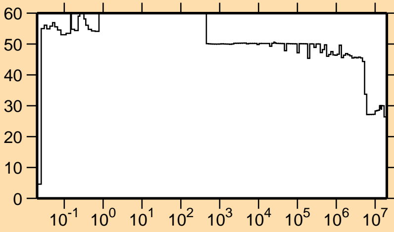
\Delta\sigma/\sigma vs. E for ^{47}\text{Ti}(n,\alpha)
