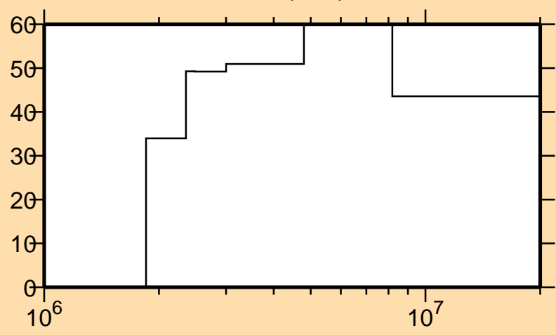
\Delta\sigma/\sigma vs. E for ^{160}\text{Gd}(n,\alpha)
