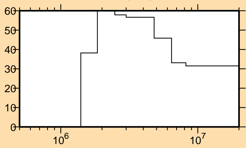
\Delta\sigma/\sigma vs. E for ^{158}\text{Gd}(n,\alpha)
