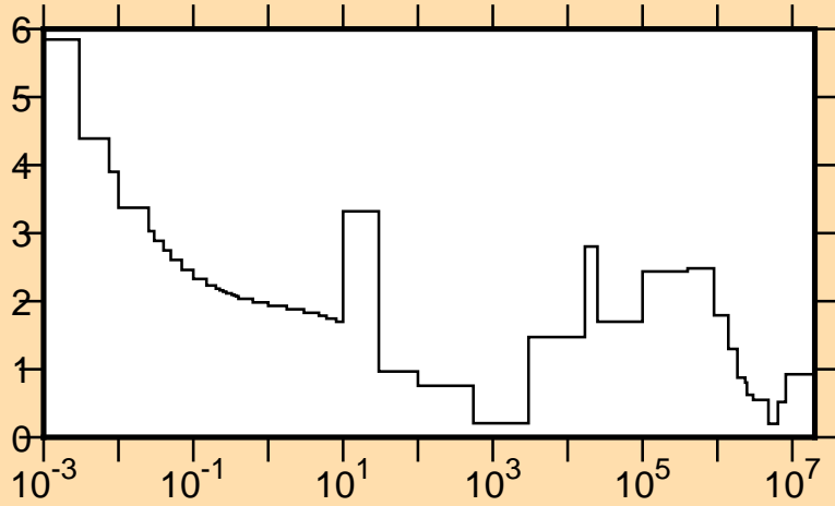
\Delta\sigma/\sigma vs. E for ^{158}\text{Gd}(n,\text{tot.})
