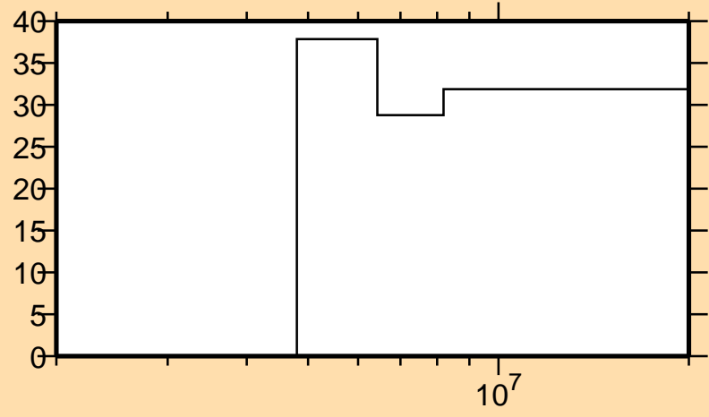
\Delta\sigma/\sigma vs. E for ^{158}\text{Gd}(n,p)
