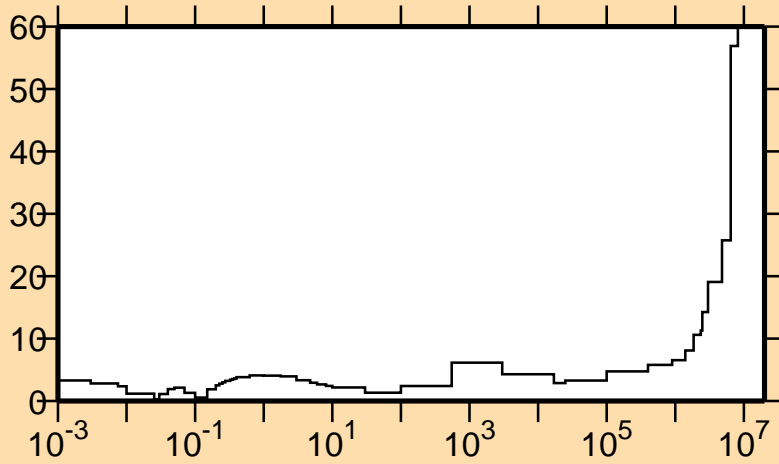
\Delta\sigma/\sigma vs. E for ^{157}\text{Gd}(n,\gamma)
