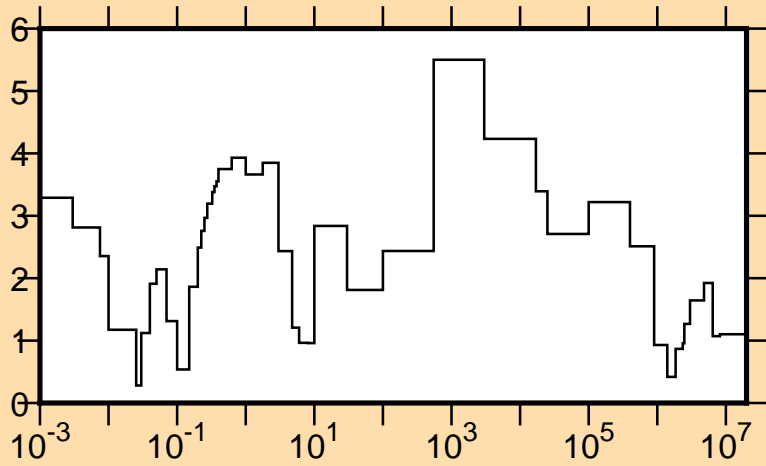
\Delta\sigma/\sigma vs. E for ^{157}\text{Gd}(n,\text{tot.})
