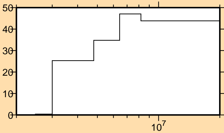
\Delta\sigma/\sigma vs. E for ^{152}\text{Gd}(n,p)
