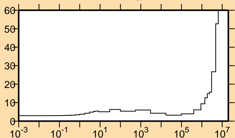
\Delta\sigma/\sigma vs. E for ^{152}\text{Gd}(n,\gamma)
