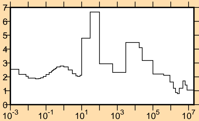
\Delta\sigma/\sigma vs. E for ^{152}\text{Gd}(n,\text{tot.})
