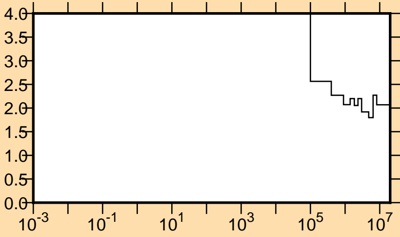
\Delta\sigma/\sigma vs. E for V(n,tot.)
