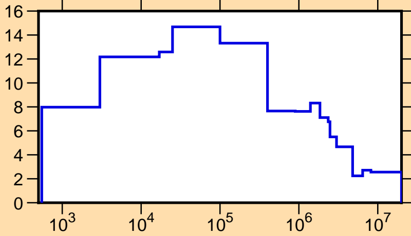
\Delta\mu/\mu vs. E for ^{255}\text{Fm}(\text{mt251})
