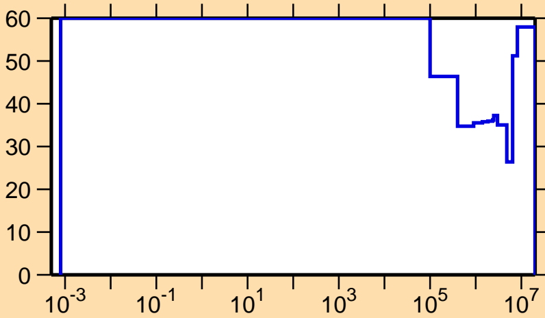
\Delta\sigma/\sigma vs. E for ^{254}\text{Es}(n,\gamma)
