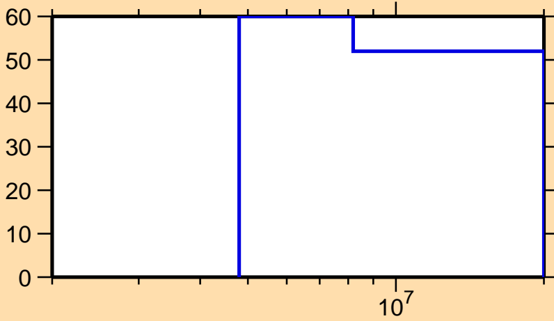
\Delta\sigma/\sigma vs. E for ^{253}\text{Es}(n,2n)
