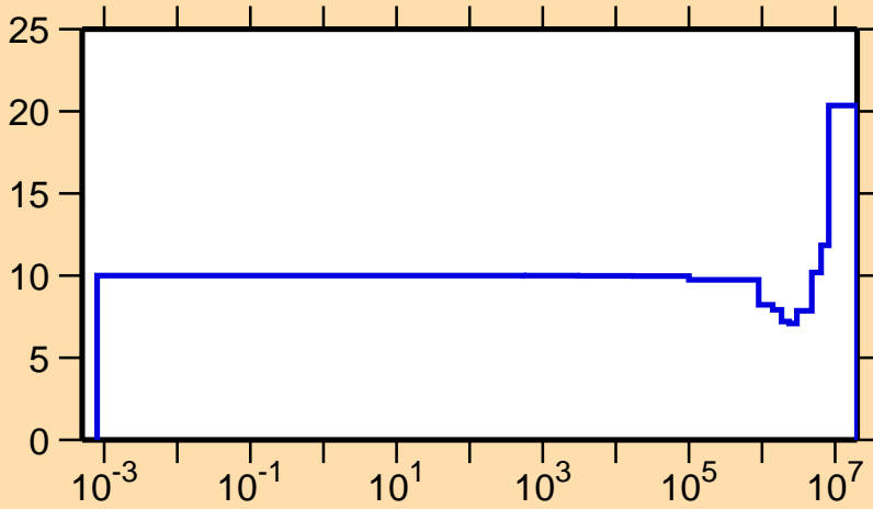
\Delta v/v vs. E for ^{254}\text{Cf}(\text{prompt } \nu)
