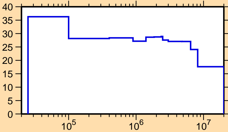
\Delta\sigma/\sigma vs. E for ^{254}\text{Cf}(n,\text{inel.})
