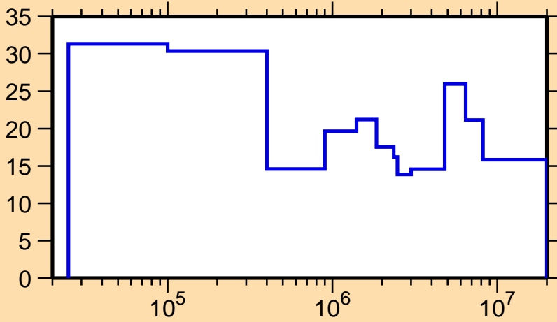
\Delta\sigma/\sigma vs. E for ^{253}\text{Cf}(n,\text{inel.})
