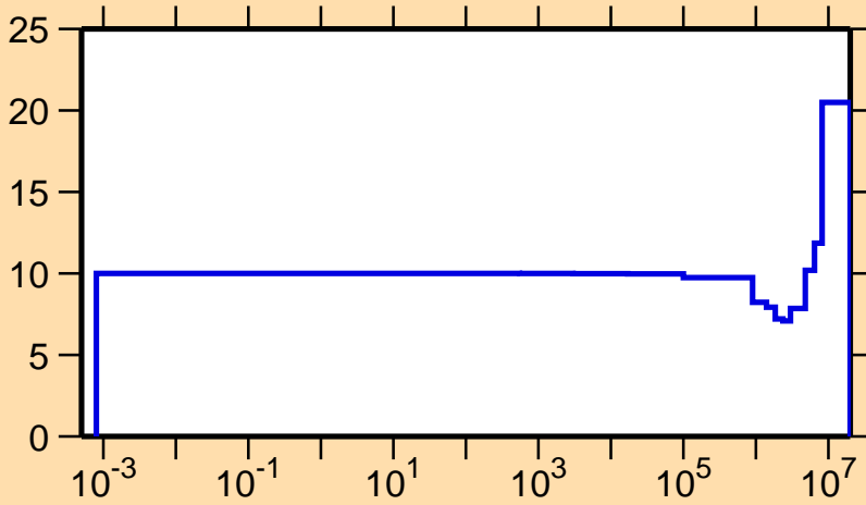
\Delta v/v vs. E for ^{253}\text{Cf} (prompt \nu )
