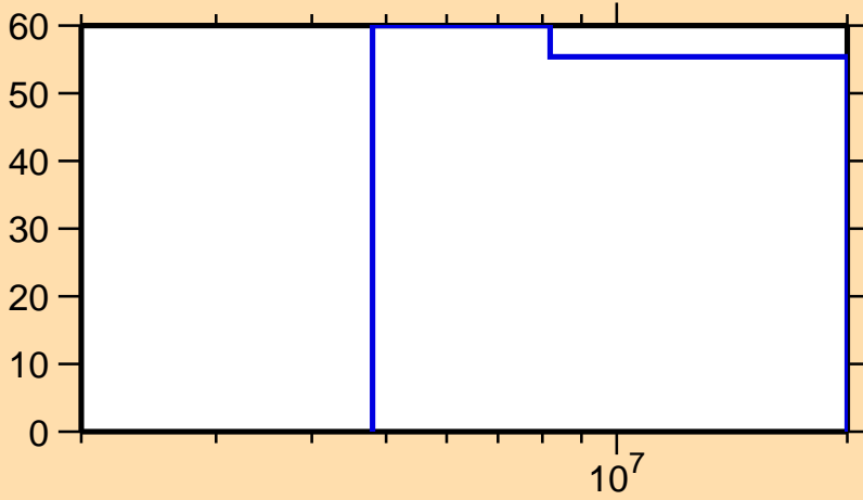
\Delta\sigma/\sigma vs. E for ^{253}\text{Cf}(n,2n)
