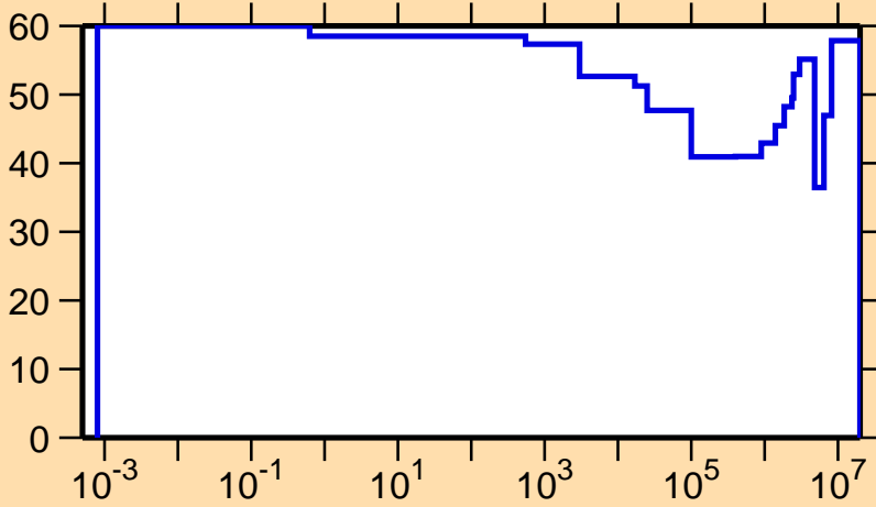
\Delta\sigma/\sigma vs. E for ^{253}\text{Cf}(n,\gamma)
