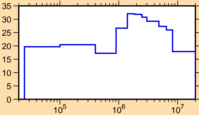
\Delta\sigma/\sigma vs. E for ^{250}\text{Cf}(n,\text{inel.})
