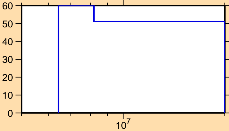
\Delta\sigma/\sigma vs. E for ^{250}\text{Cf}(n,2n)
