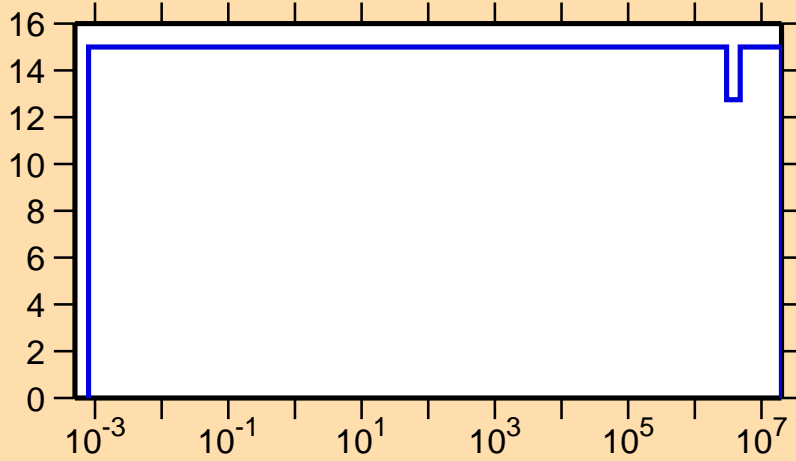
\Delta v/v vs. E for ^{248}\text{Cf}(\text{delayed } \nu)
