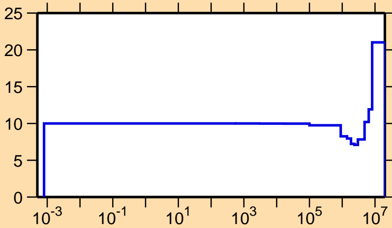
\Delta v/v vs. E for ^{248}\text{Cf}(\text{prompt } \nu)
