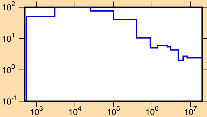
\Delta\mu/\mu vs. E for ^{250}\text{Bk}(\text{mt251})
