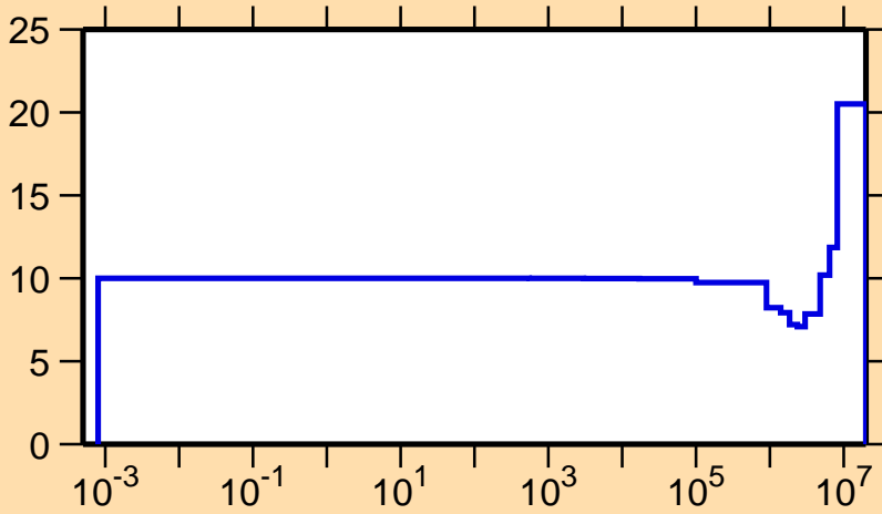
\Delta v/v vs. E for ^{250}\text{Bk} (prompt \nu )
