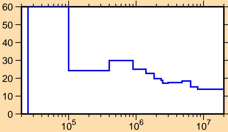
\Delta\sigma/\sigma vs. E for ^{250}\text{Bk}(n,\text{inel.})
