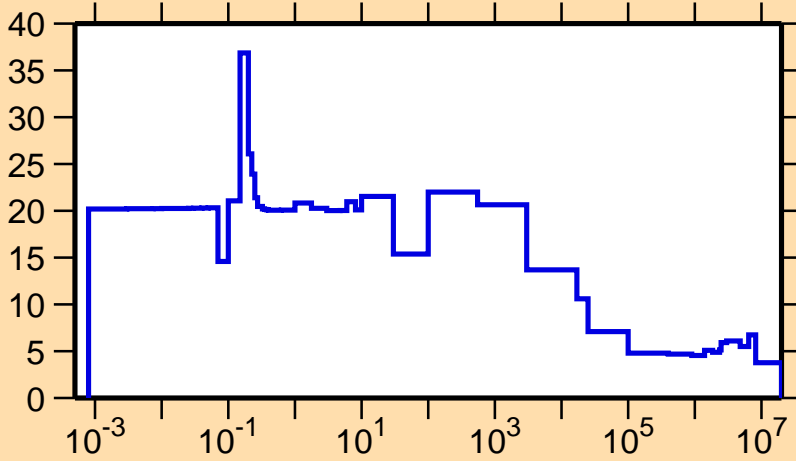
\Delta\sigma/\sigma vs. E for ^{249}\text{Bk}(n,\text{el.})
