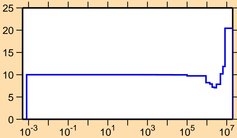
\Delta v/v vs. E for ^{249}\text{Bk}(\text{prompt } \nu)
