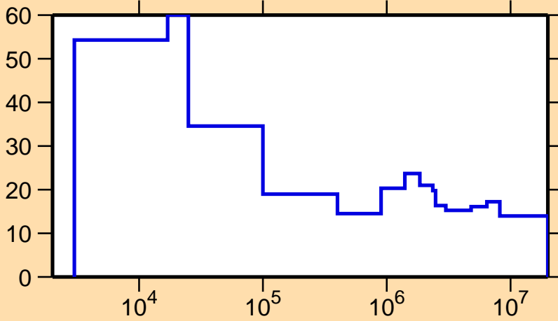
\Delta\sigma/\sigma vs. E for ^{249}\text{Bk}(n,\text{inel.})
