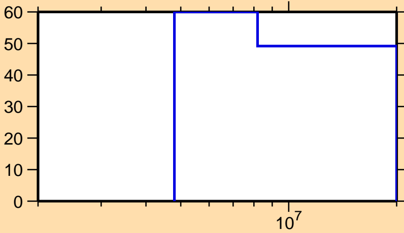
\Delta\sigma/\sigma vs. E for ^{248}\text{Bk}(n,2n)
