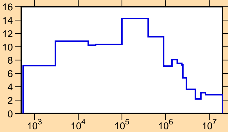
\Delta\mu/\mu vs. E for ^{248}\text{Bk}(\text{mt251})
