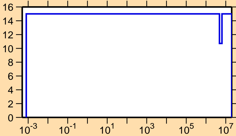
\Delta v/v vs. E for ^{248}\text{Bk} (delayed \nu )
