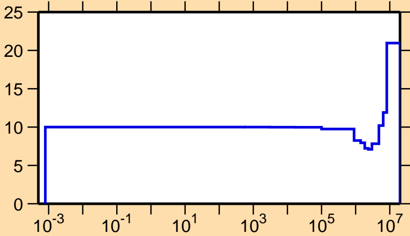
\Delta v/v vs. E for ^{248}\text{Bk}(\text{prompt } \nu)
