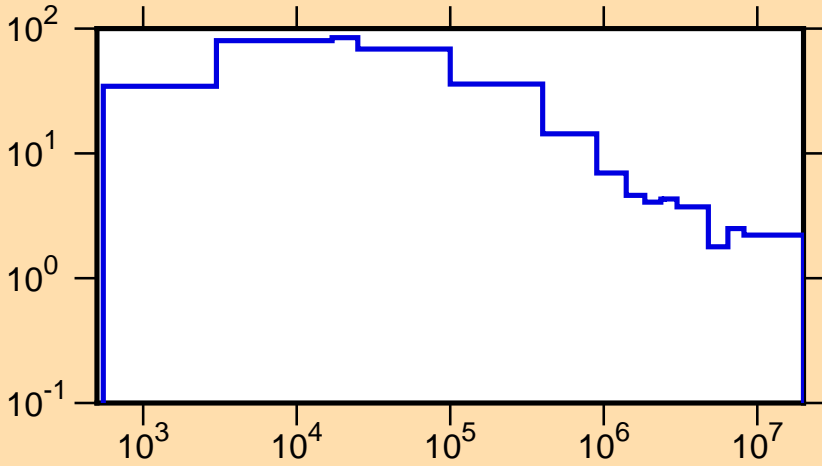
\Delta\mu/\mu vs. E for ^{247}\text{Bk}(\text{mt251})
