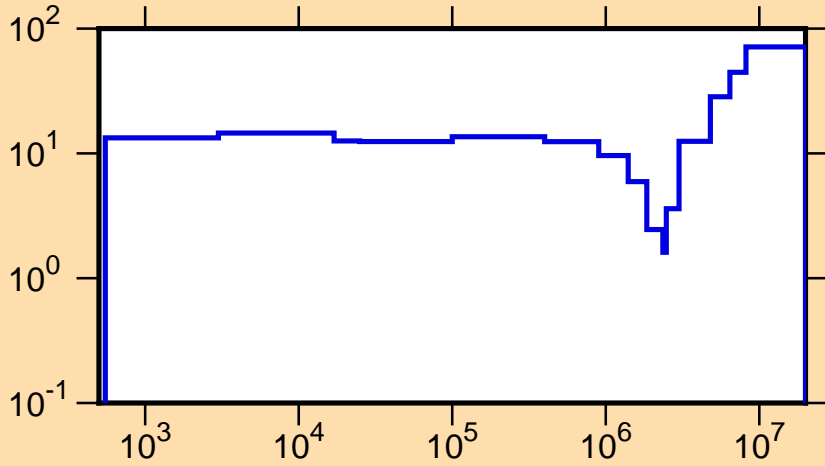
\Delta\phi/\phi vs. E for ^{247}\text{Bk}(n,f)
