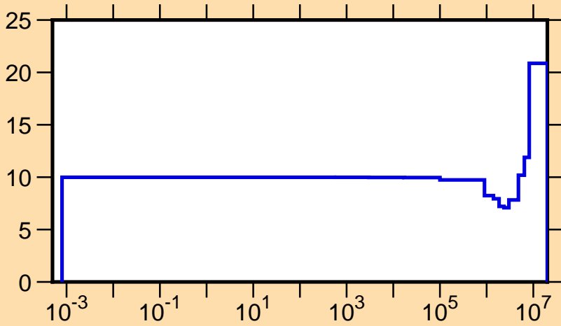
\Delta v/v vs. E for ^{247}\text{Bk}(\text{total } \nu)
