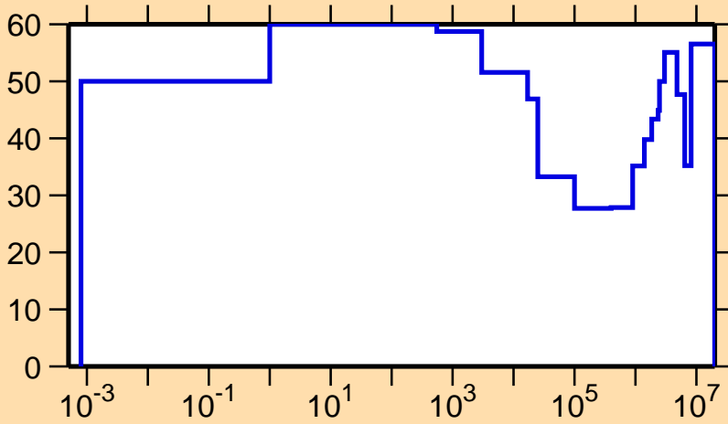
\Delta\sigma/\sigma vs. E for ^{247}\text{Bk}(n,\gamma)
