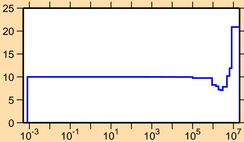
\Delta v/v vs. E for ^{247}\text{Bk}(\text{prompt } \nu)
