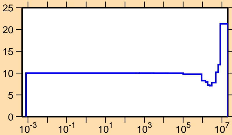
\Delta v/v vs. E for ^{245}\text{Bk}(\text{prompt } \nu)
