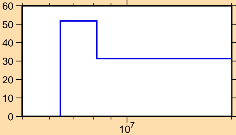
\Delta\sigma/\sigma vs. E for ^{246}\text{Cm}(n,2n)
