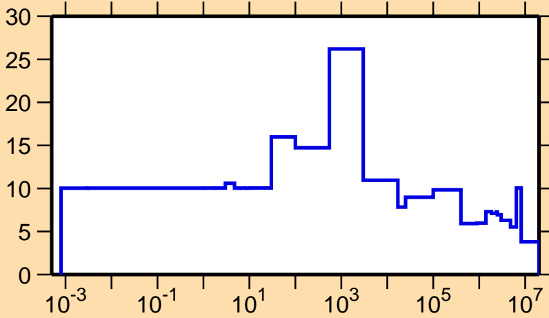
\Delta\sigma/\sigma vs. E for ^{246}\text{Cm}(n,\text{el.})
