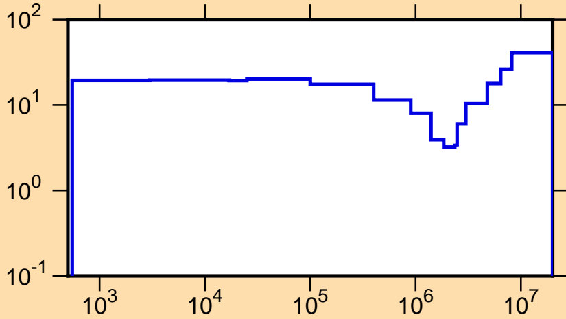
\Delta\phi/\phi vs. E for ^{243}\text{Cm}(n,f)
