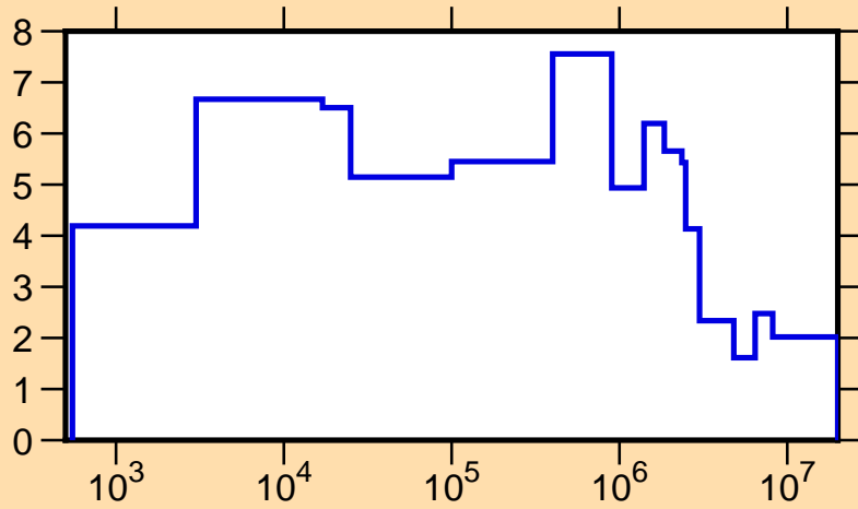
\Delta\mu/\mu vs. E for ^{243}\text{Cm}(\text{mt251})
