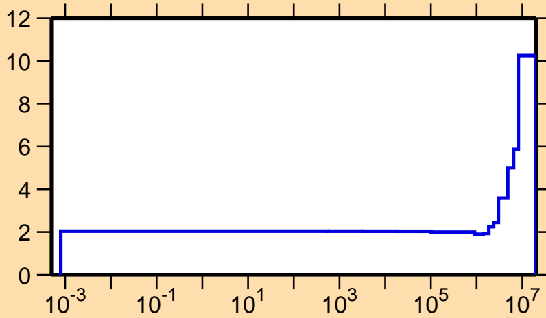
\Delta v/v vs. E for ^{243}\text{Cm} (prompt \nu )
