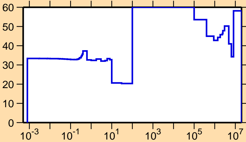
\Delta\sigma/\sigma vs. E for ^{243}\text{Cm}(n,\gamma)
