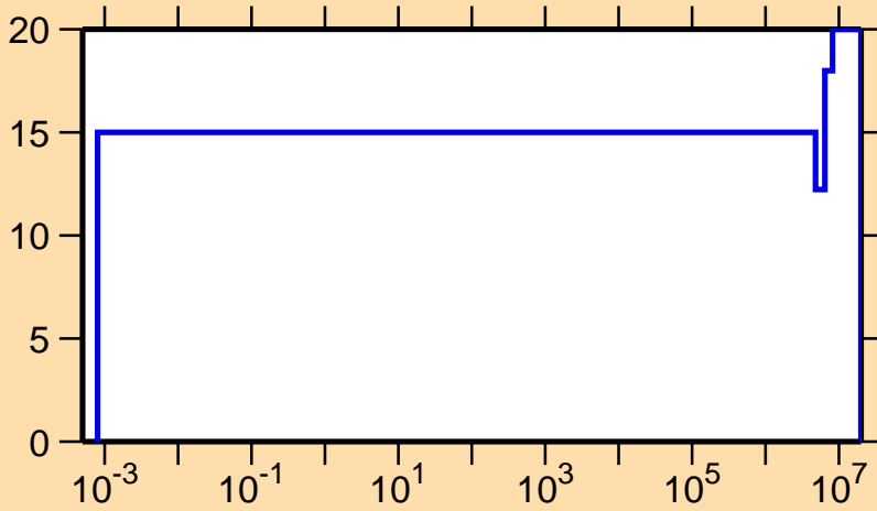
\Delta v/v vs. E for ^{243}\text{Cm} (delayed \nu )
