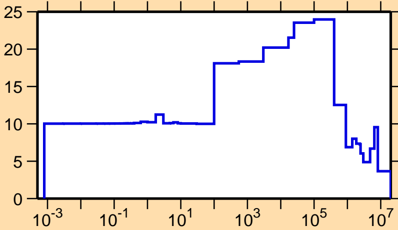
\Delta\sigma/\sigma vs. E for ^{243}\text{Cm}(n,\text{el.})
