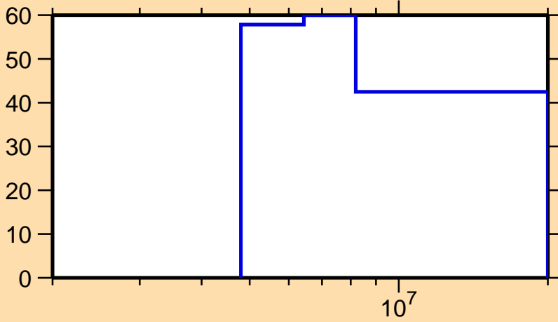
\Delta\sigma/\sigma vs. E for ^{243}\text{Cm}(n,2n)
