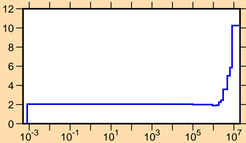
\Delta v/v vs. E for ^{243}\text{Cm} (total v )
