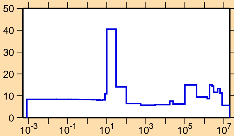
\Delta\sigma/\sigma vs. E for ^{242}\text{Cm}(n,f)
