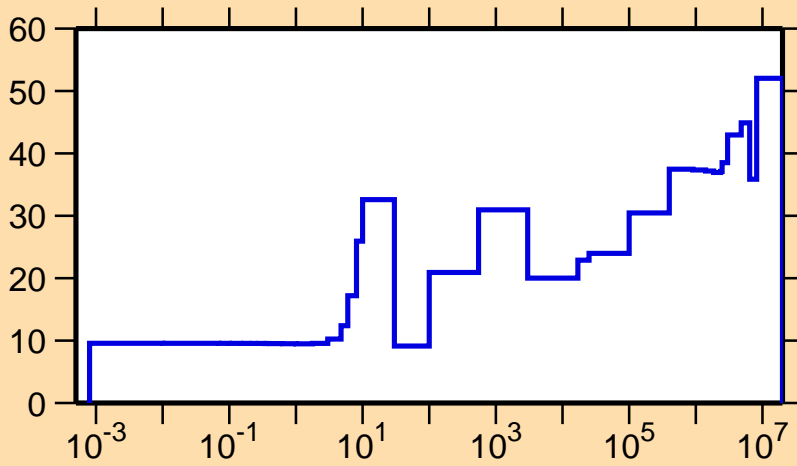
\Delta\sigma/\sigma vs. E for ^{242}\text{Cm}(n,\gamma)
