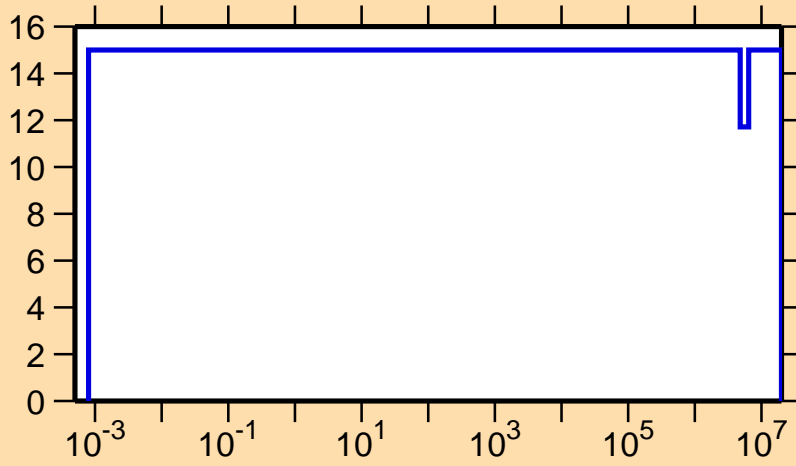
\Delta\nu/\nu vs. E for ^{240}\text{Cm} (delayed \nu )
