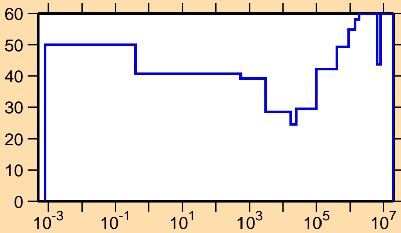
\Delta\sigma/\sigma vs. E for ^{239}\text{Np}(n,\gamma)
