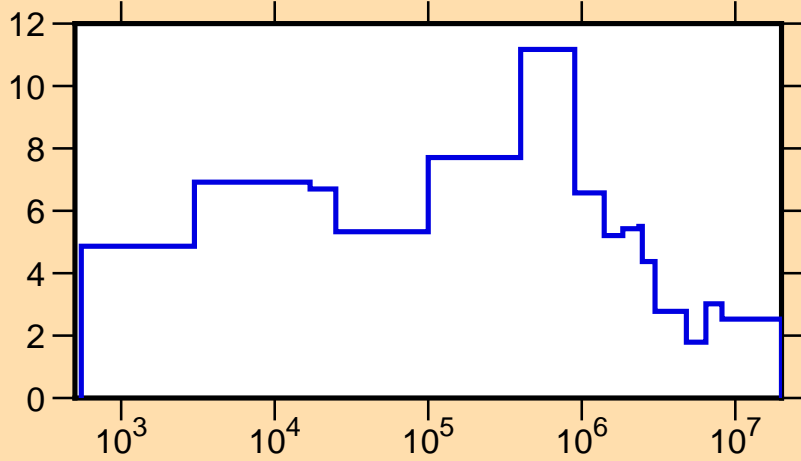
\Delta\mu/\mu vs. E for ^{239}\text{Np}(\text{mt251})
