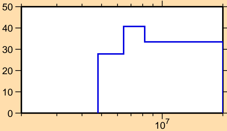
\Delta\sigma/\sigma vs. E for ^{238}\text{Np}(n,2n)
