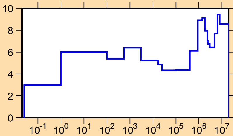
\Delta\sigma/\sigma vs. E for ^{237}\text{Np}(n,\text{el.})
