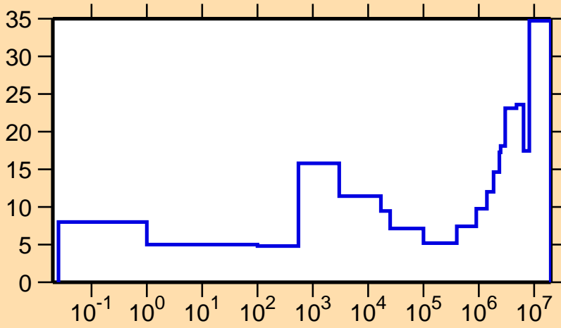
\Delta\sigma/\sigma vs. E for ^{237}\text{Np}(n,\gamma)
