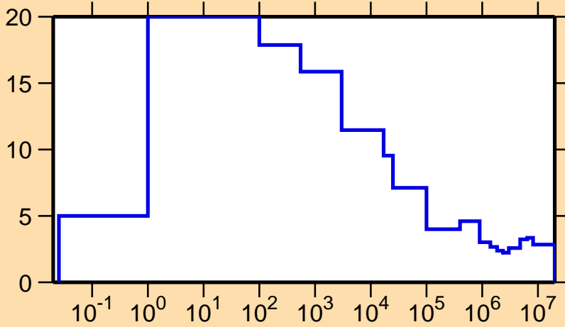
\Delta\sigma/\sigma vs. E for ^{237}\text{Np}(n,f)
