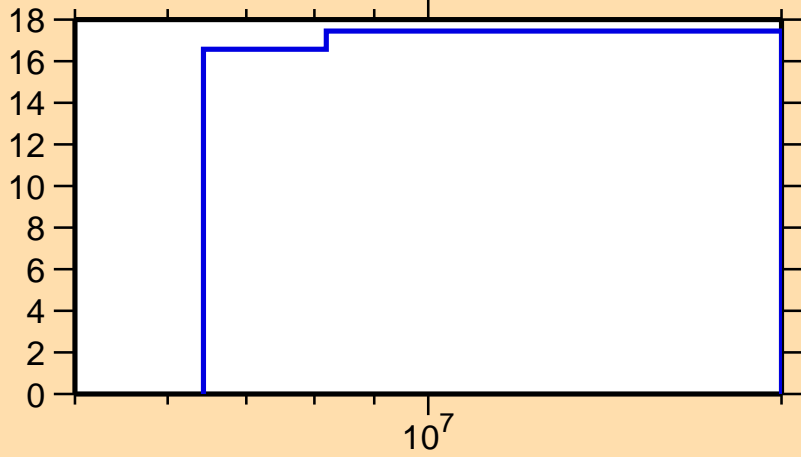
\Delta\sigma/\sigma vs. E for ^{236}\text{U}(n,2n)
