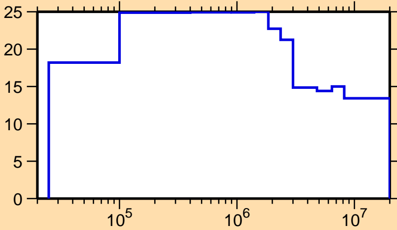
\Delta\sigma/\sigma vs. E for ^{236}\text{U}(n,\text{inel.})
