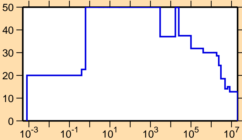
\Delta\sigma/\sigma vs. E for ^{236}\text{U}(n,f)
