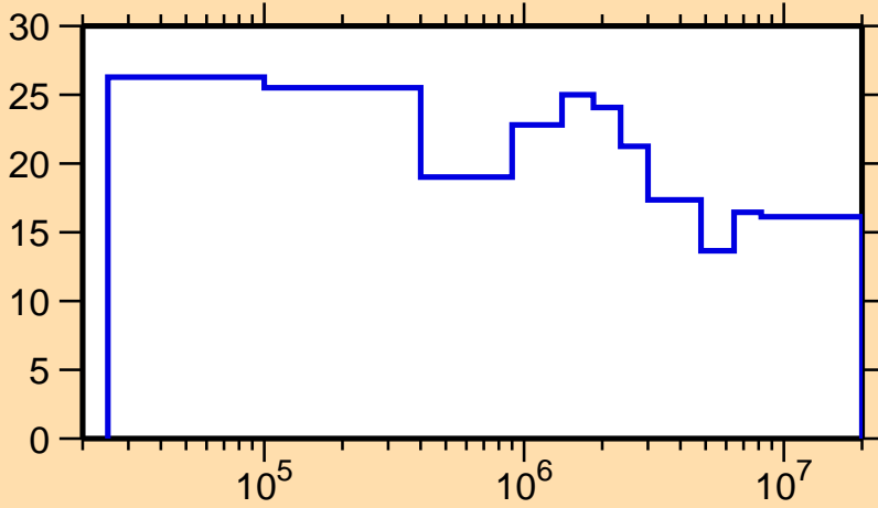
\Delta\sigma/\sigma vs. E for ^{234}\text{U}(n,\text{inel.})
