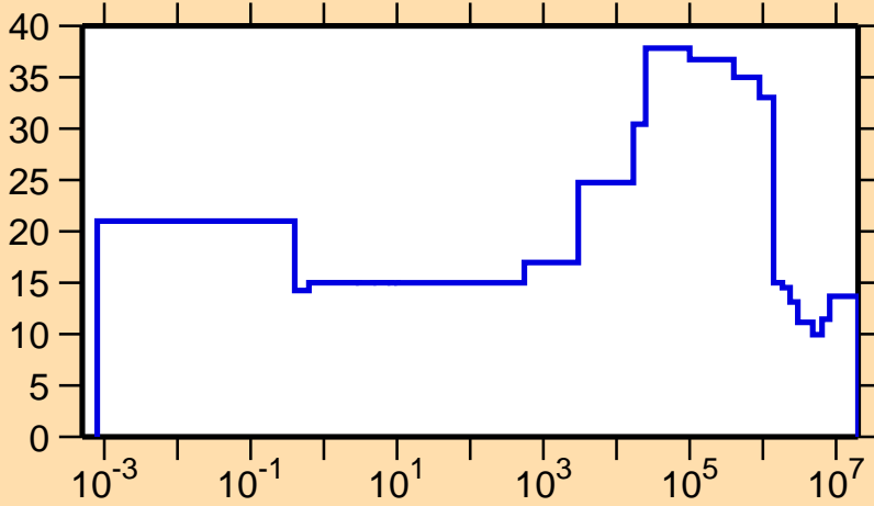
\Delta\sigma/\sigma vs. E for ^{234}\text{U}(n,f)
