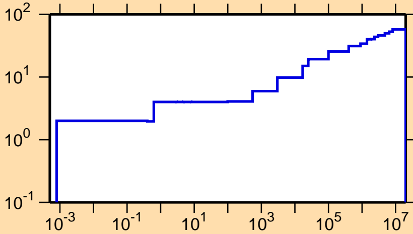
\Delta\sigma/\sigma vs. E for ^{234}\text{U}(n,\gamma)
