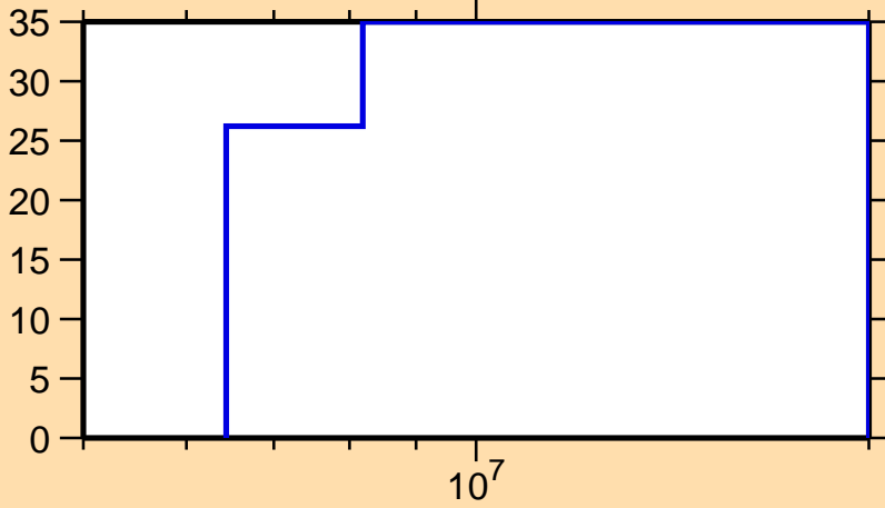
\Delta\sigma/\sigma vs. E for ^{234}\text{U}(n,2n)
