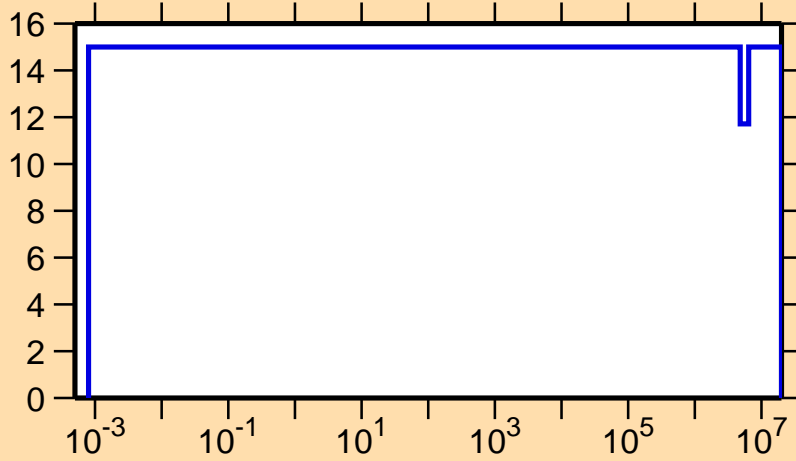
\Delta\nu/\nu vs. E for ^{234}\text{Th} (delayed \nu )
