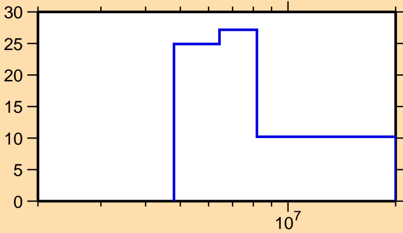
\Delta\sigma/\sigma vs. E for ^{234}\text{Th}(n,2n)
