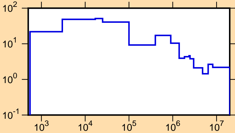
\Delta\mu/\mu vs. E for ^{234}\text{Th}(\text{mt251})
