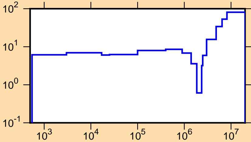
\Delta\phi/\phi vs. E for ^{234}\text{Th}(n,f)
