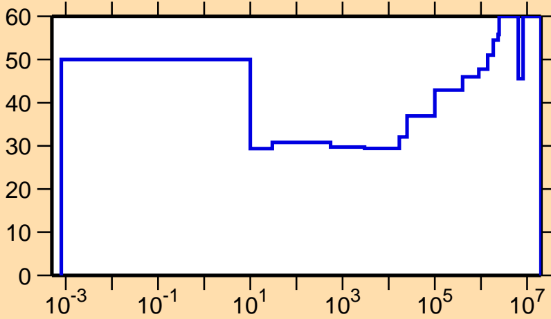
\Delta\sigma/\sigma vs. E for ^{234}\text{Th}(n,\gamma)
