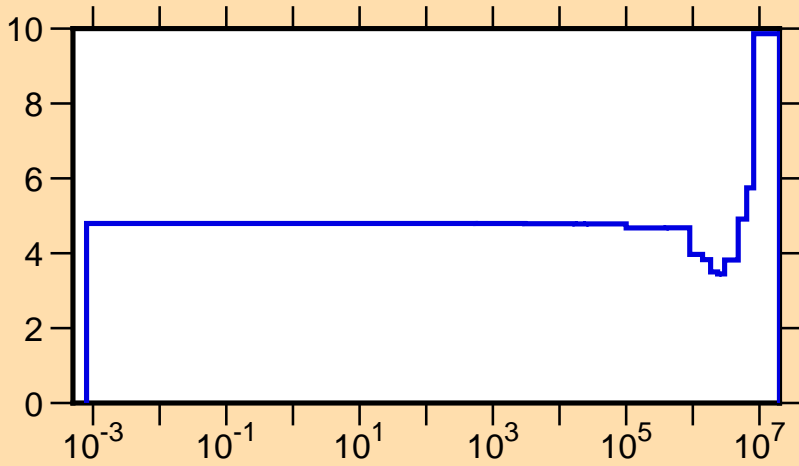
\Delta v/v vs. E for ^{234}\text{Th}(\text{total } \nu)
