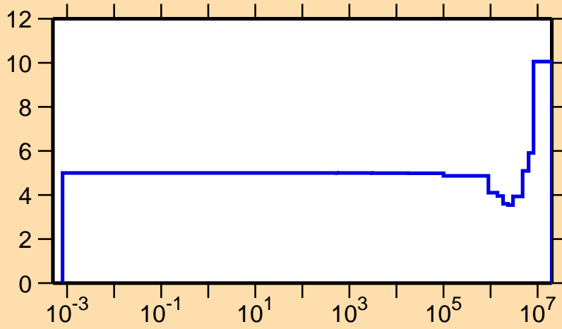
\Delta v/v vs. E for ^{234}\text{Th} (prompt \nu )
