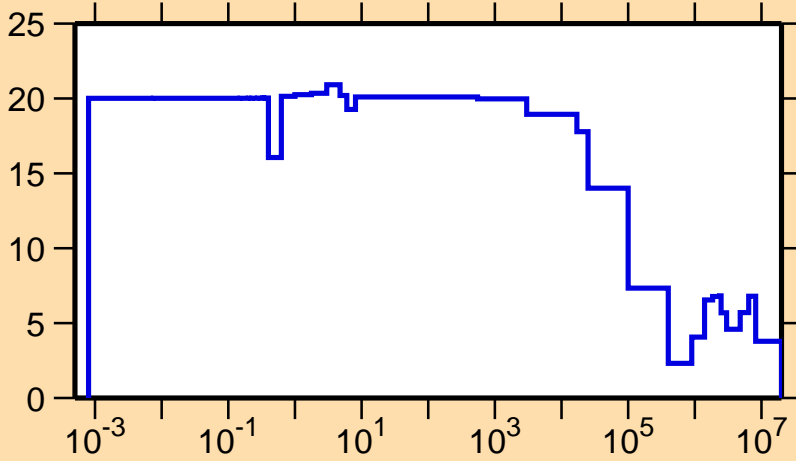
\Delta\sigma/\sigma vs. E for ^{229}\text{Th}(n,\text{el.})
