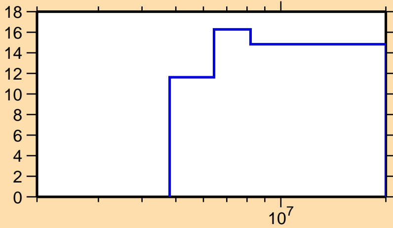
\Delta\sigma/\sigma vs. E for ^{229}\text{Th}(n,2n)
