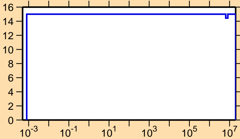
\Delta v/v vs. E for ^{229}\text{Th} (delayed \nu )
