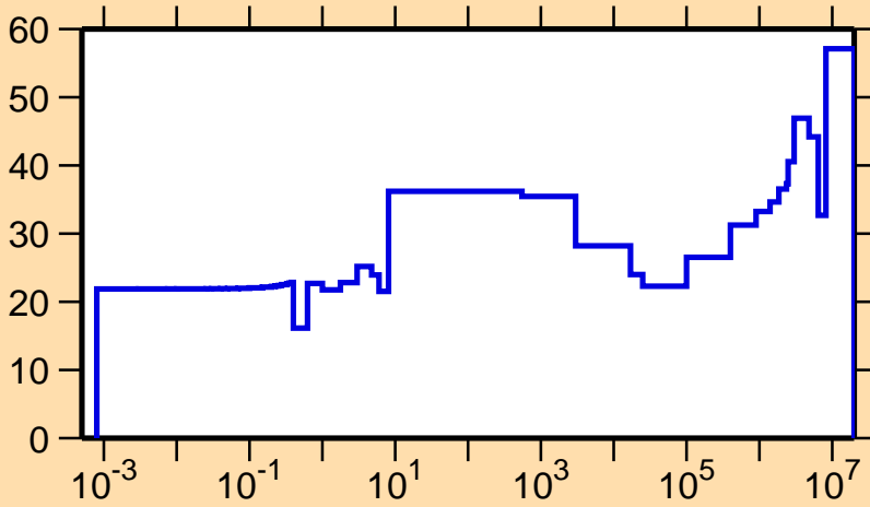
\Delta\sigma/\sigma vs. E for ^{229}\text{Th}(n,\gamma)
