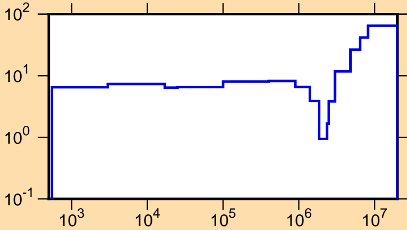
\Delta\phi/\phi vs. E for ^{229}\text{Th}(n,f)
