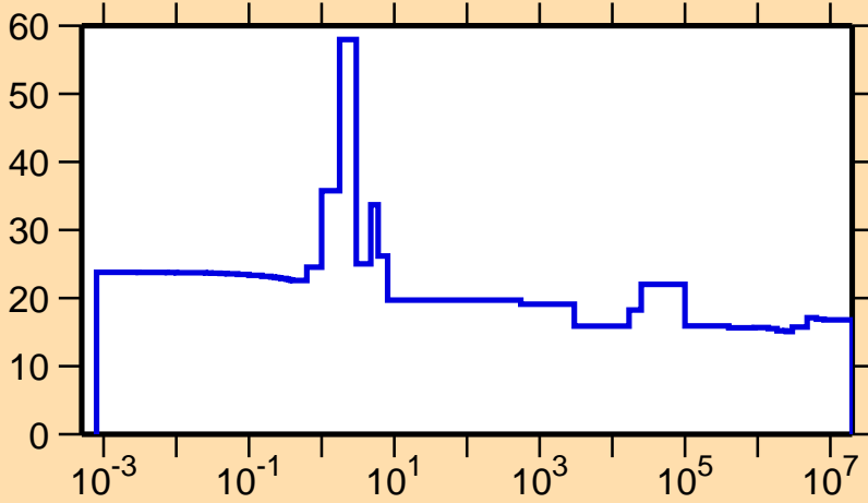
\Delta\sigma/\sigma vs. E for ^{229}\text{Th}(n,f)
