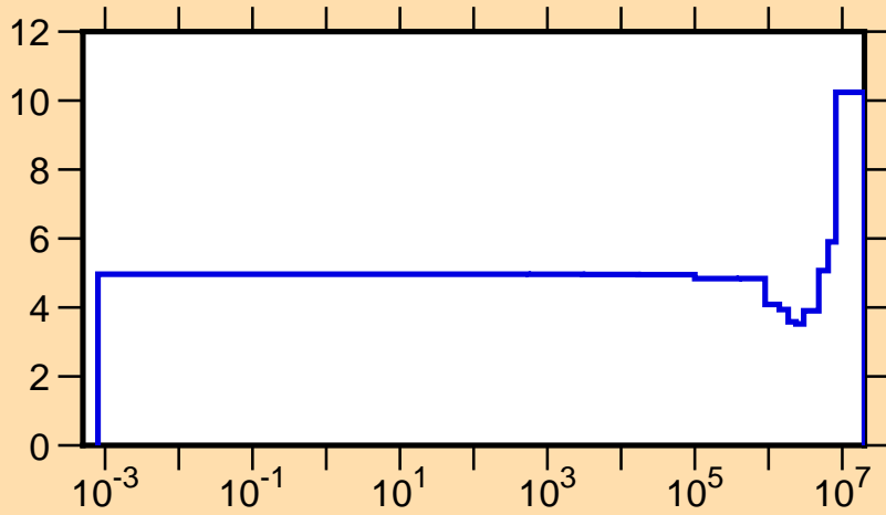
\Delta v/v vs. E for ^{229}\text{Th}(\text{total } \nu)
