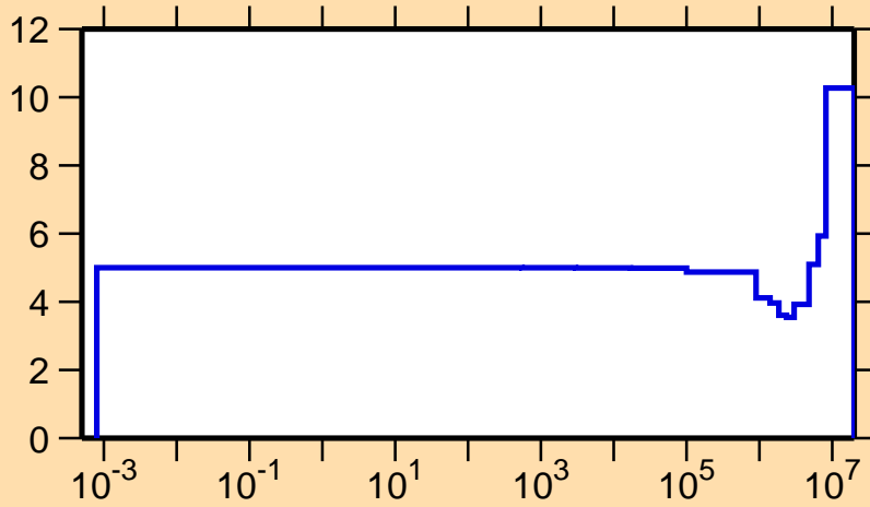
\Delta v/v vs. E for ^{229}\text{Th} (prompt \nu )
