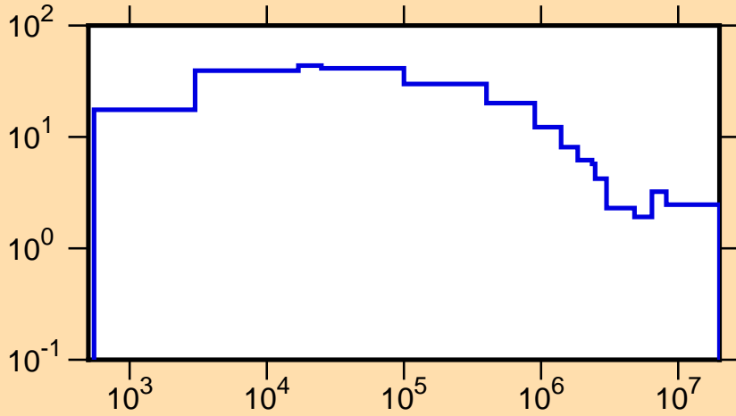
\Delta\mu/\mu vs. E for ^{229}\text{Th}(\text{mt251})
