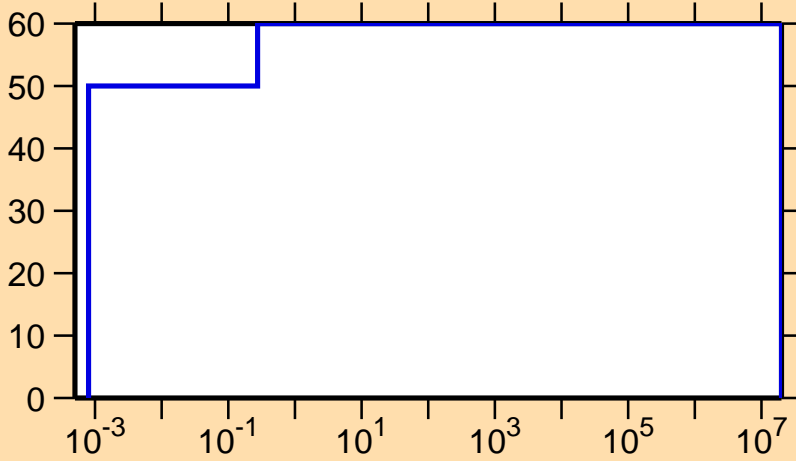
\Delta\sigma/\sigma vs. E for ^{226}\text{Ac}(n,f)
