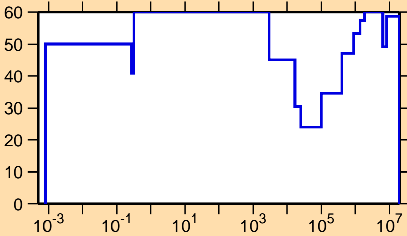
\Delta\sigma/\sigma vs. E for ^{226}\text{Ac}(n,\gamma)
