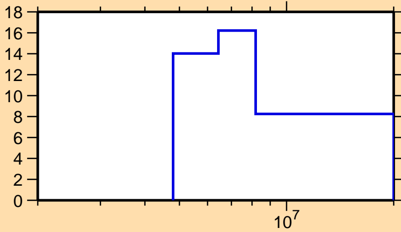
\Delta\sigma/\sigma vs. E for ^{226}\text{Ac}(n,2n)
