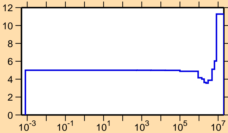
\Delta v/v vs. E for ^{226}\text{Ac}(\text{prompt } \nu)
