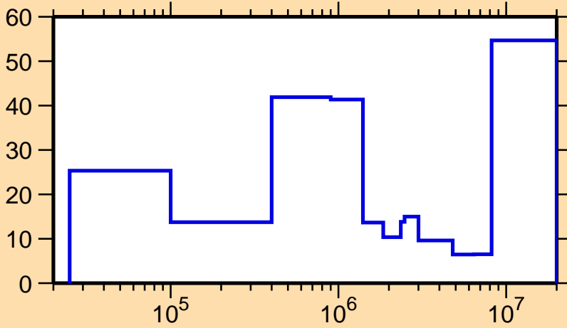
\Delta\sigma/\sigma vs. E for ^{193}\text{Ir}(n,\text{inel.})
