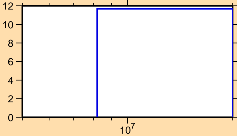
\Delta\sigma/\sigma vs. E for ^{191}\text{Ir}(n,2n)
