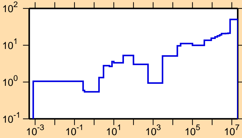
\Delta\sigma/\sigma vs. E for ^{191}\text{Ir}(n,\gamma)
