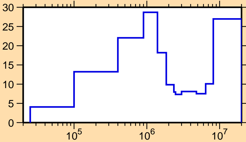
\Delta\sigma/\sigma vs. E for ^{191}\text{Ir}(n,\text{inel.})
