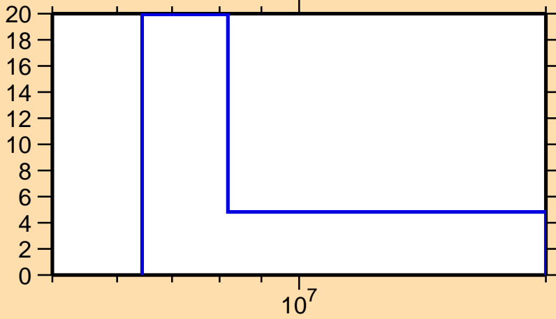
\Delta\sigma/\sigma vs. E for ^{170}\text{Er}(n,2n)
