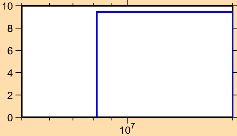
\Delta\sigma/\sigma vs. E for ^{156}\text{Gd}(n,2n)
