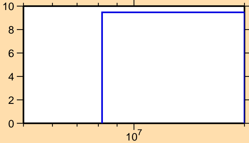
\Delta\sigma/\sigma vs. E for ^{154}\text{Gd}(n,2n)
