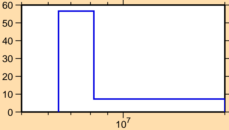
\Delta\sigma/\sigma vs. E for ^{153}\text{Gd}(n,2n)
