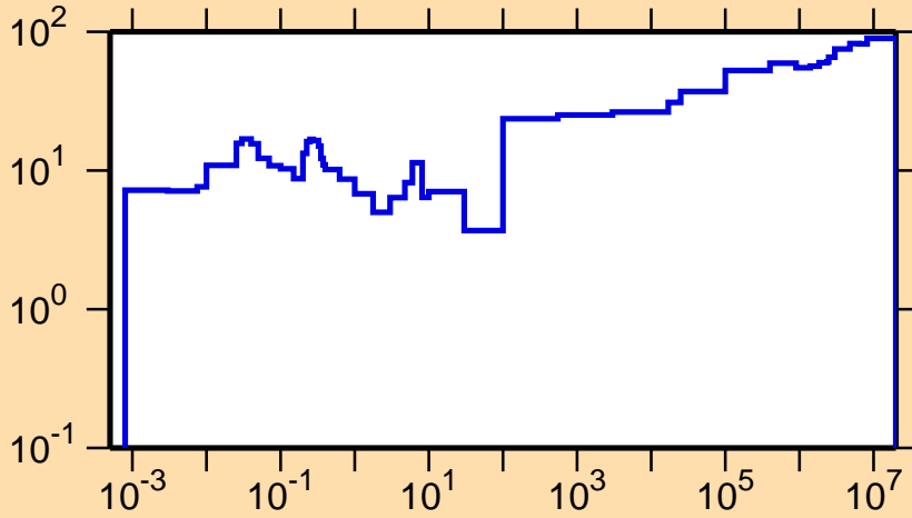
\Delta\sigma/\sigma vs. E for ^{153}\text{Gd}(n,\gamma)
