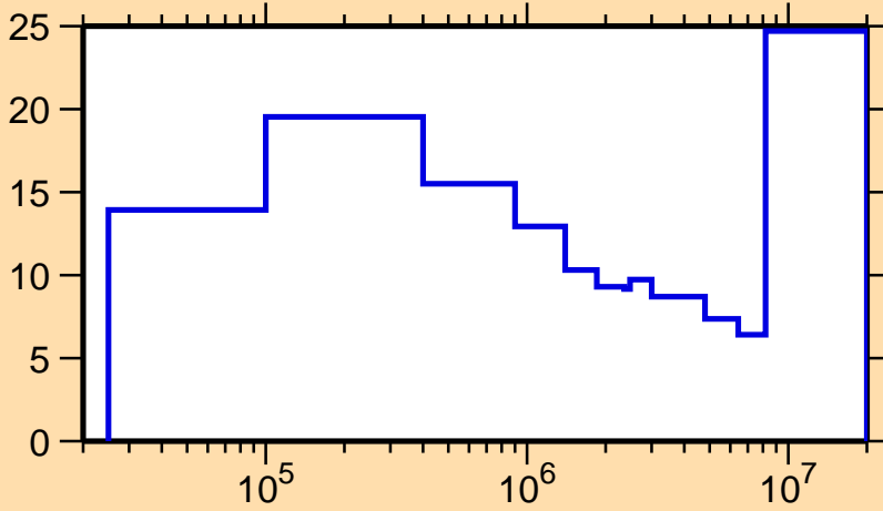
\Delta\sigma/\sigma vs. E for ^{153}\text{Gd}(n,\text{inel.})
