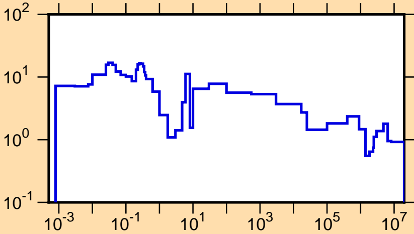
\Delta\sigma/\sigma vs. E for ^{153}\text{Gd}(n,\text{tot.})
