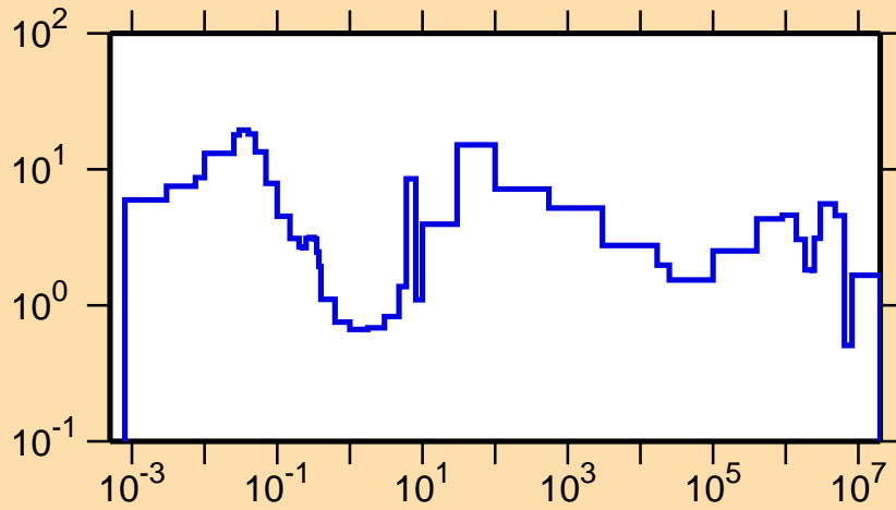
\Delta\sigma/\sigma vs. E for ^{153}\text{Gd}(n,\text{el.})
