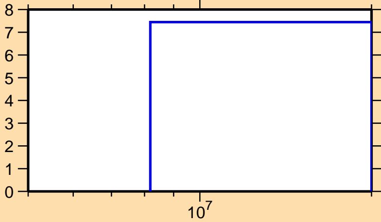
\Delta\sigma/\sigma vs. E for ^{155}\text{Eu}(n,2n)
