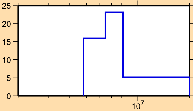
\Delta\sigma/\sigma vs. E for ^{149}\text{Sm}(n,2n)
