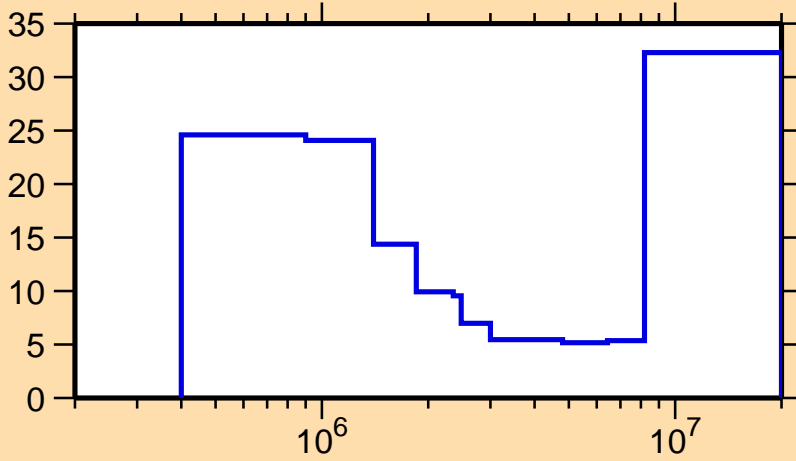
\Delta\sigma/\sigma vs. E for ^{146}\text{Nd}(n,\text{inel.})
