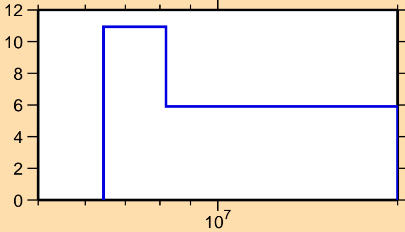
\Delta\sigma/\sigma vs. E for ^{146}\text{Nd}(n,2n)
