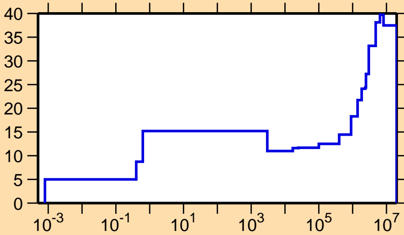
\Delta\sigma/\sigma vs. E for ^{145}\text{Nd}(n,\gamma)
