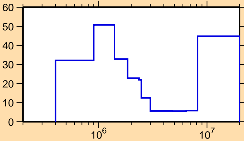
\Delta\sigma/\sigma vs. E for ^{143}\text{Nd}(n,\text{inel.})
