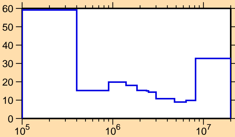
\Delta\sigma/\sigma vs. E for ^{135}\text{Cs}(n,\text{inel.})
