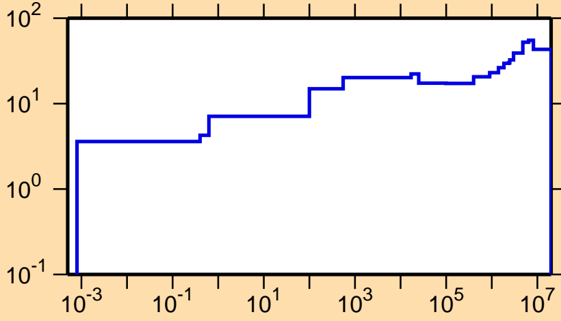
\Delta\sigma/\sigma vs. E for ^{135}\text{Cs}(n,\gamma)
