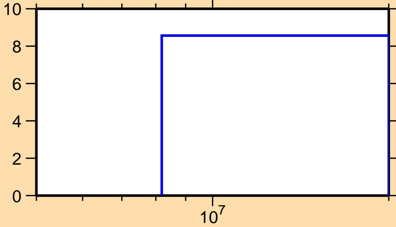
\Delta\sigma/\sigma vs. E for ^{135}\text{Cs}(n,2n)
