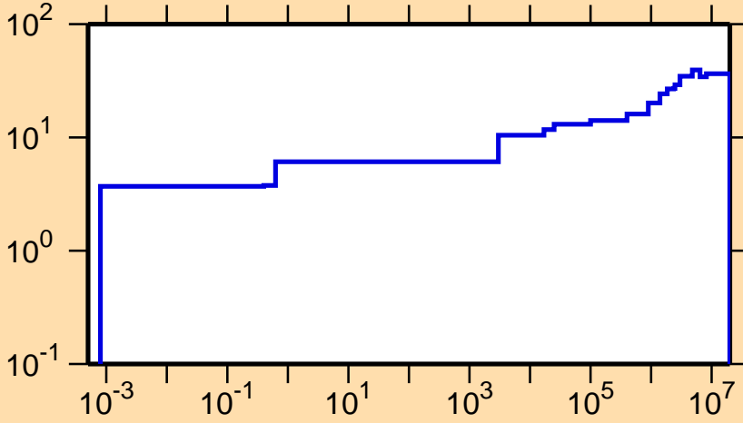
\Delta\sigma/\sigma vs. E for ^{133}\text{Cs}(n,\gamma)
