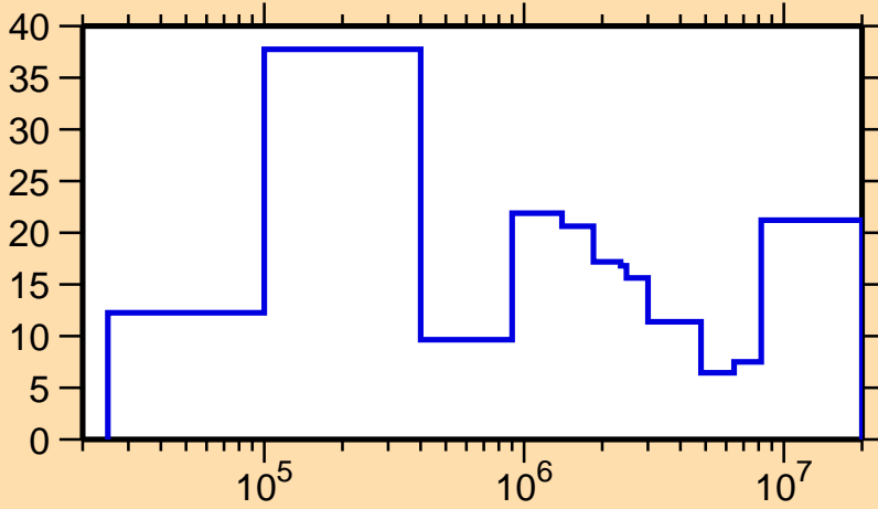
\Delta\sigma/\sigma vs. E for ^{133}\text{Cs}(n,\text{inel.})
