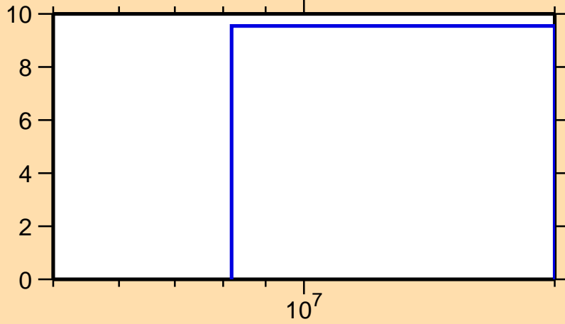
\Delta\sigma/\sigma vs. E for ^{133}\text{Cs}(n,2n)
